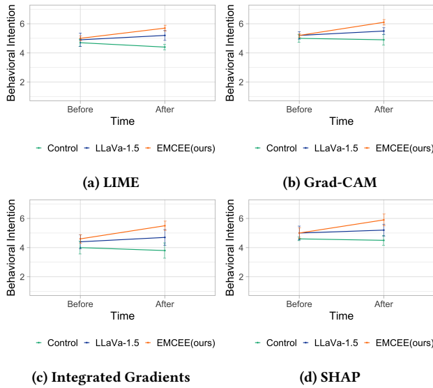
Figure 18: Participants' self-report behavioral intention score for (a) LIME and (b) Grad-CAM (c) Integrated Gradients (d) SHAP before and after conditions.
